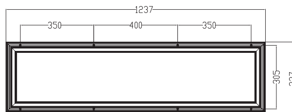
enl-CP650-30-xyy-1237
